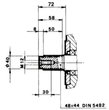
90005 Macho 48X44 Z-23T
